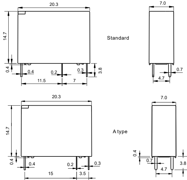
Outline dimensions
