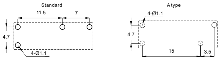
PCB board layout (Bottom view)
